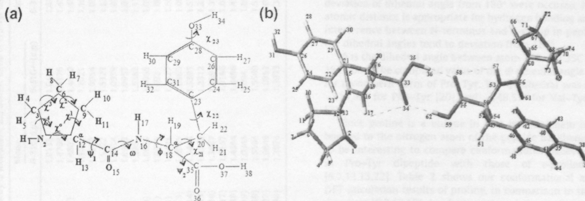
Fig. 1. The molecular model of neutral L-Pro-Tyr dipeptide (a). Atom numbering and dihedral angles were shown. The global conformation of dimeric form of Pro-Tyr dipeptide (b). Predicted H-bonding interactions are shown as broken lines.
