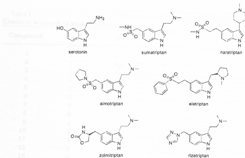
FIG. 1 Structures of some agonists for 5-HT 1D receptor
