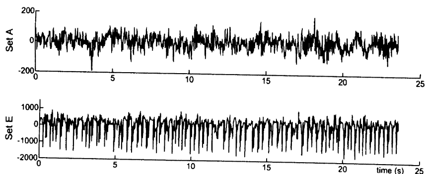
Fig. 1. EEG examples for two different sets: set A (healthy) and set E (epileptic).
